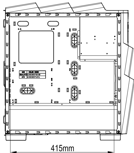
Maximum VGA Card Length:415mm
