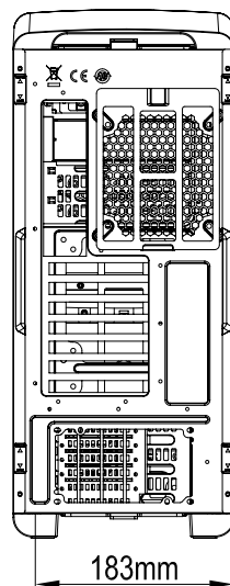
Maximum CPU Cooler Height:183mm
